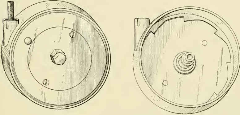
Fig. 109. Form of Trolley Catcher with Drum and Reel
